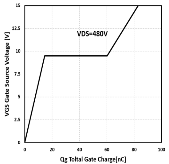
Figure4: Typical gate charge VS. V_{GS} , I_C=40\text{A}
