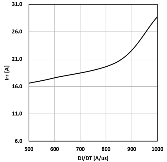
Figure 14. Typical diode Irr vs di/dt Tc=25°C VCE=400V VGE=15V IF=40A
