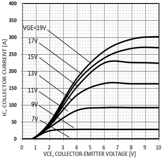
Figure 5. Typical output characteristics t_p=300\mu s T_c=25^\circ C
