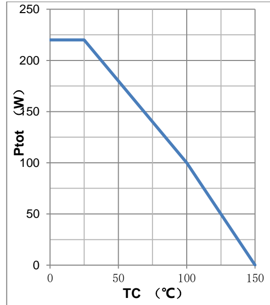
Figure2:power dissipation VS. case temprature
